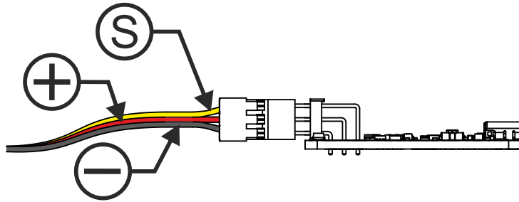
Way to connect the servos.
