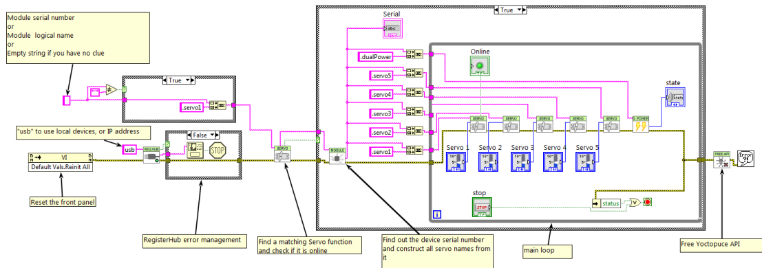
Example of Yocto-Servo-C usage in LabVIEW
