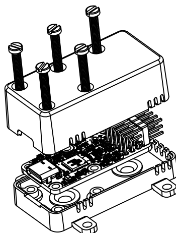
You can install your Yocto-Servo-C in an optional enclosure
