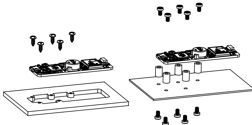
Examples of assembly on supports
