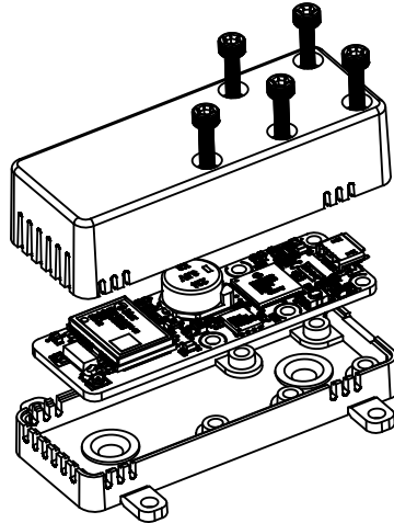
You can install your Yocto-GPS-V2 in an optional enclosure
