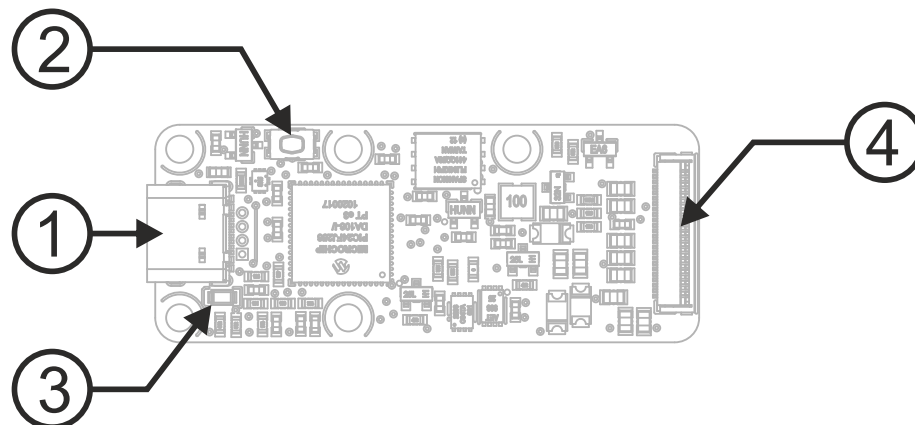
1: Type-C USB socket 3: Yocto-led 2: Yocto-button 4: ZIF connector
