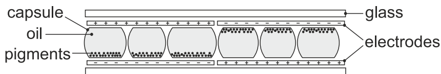
Simplified diagram of the internal structure of an electrophoretic display
