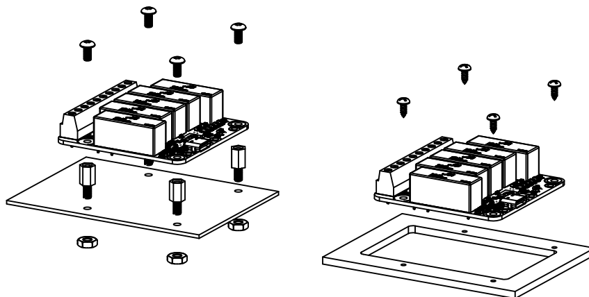
Examples of assembly on supports
