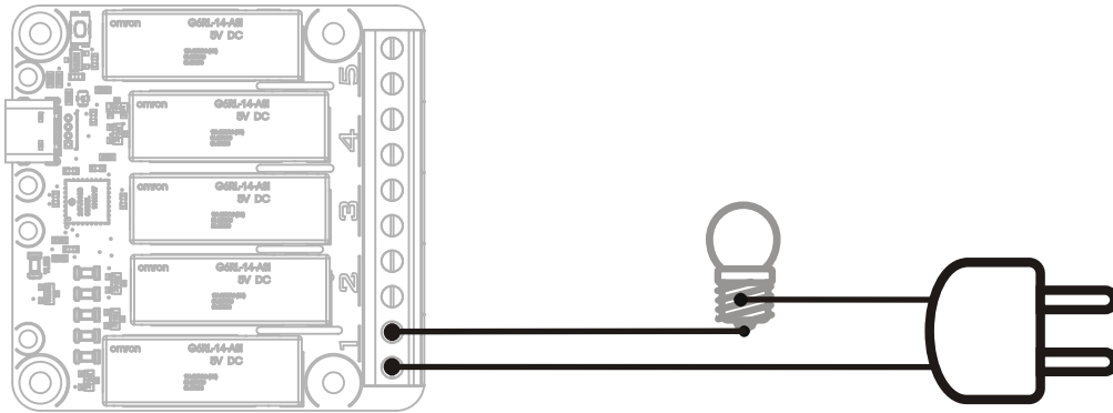
Pilot a light bulb with your Yocto-MaxiPowerRelay-C module.
