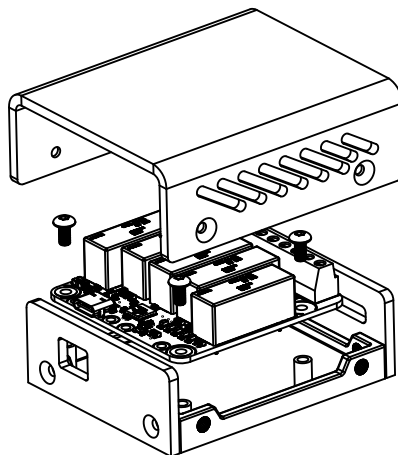
You can install your Yocto-MaxiPowerRelay-C in an optional enclosure
