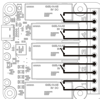
Relay wiring inside the module.
