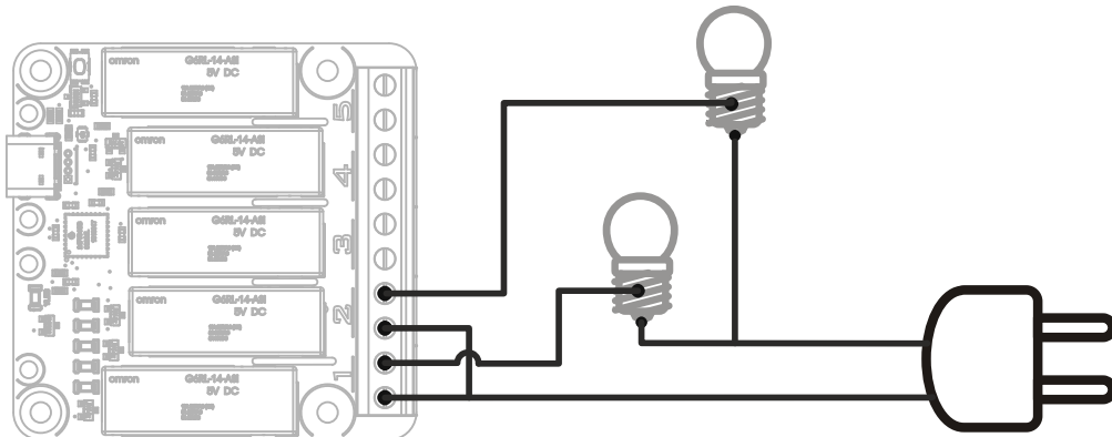
Pilot two light bulbs with your Yocto-MaxiPowerRelay-C module.
