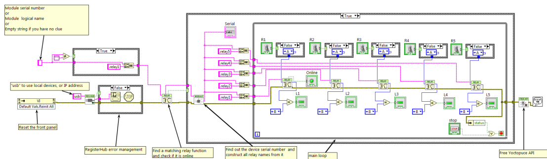
Example of Yocto-MaxiPowerRelay-C usage in LabVIEW
